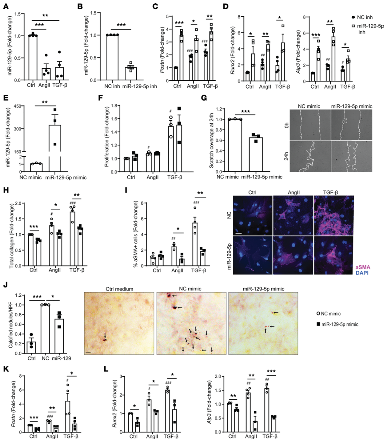
Figure 3. miR-129-5p inhibits both CF-to-MF and CF-to-OF transition. (A) miR-129-5p expression in CF upon AngII or TGF- \beta stimulation as assessed by qPCR. (B) miR-129-5p expression in CF upon miR-129-5p inhibition as assessed by qPCR. (C and D) AngII- and TGF- \beta -induced expression of Postn , Runx2 , and Alp3 transcripts in CF upon miR-129-5p inhibition as assessed by qPCR. (E) miR-129-5p expression in CF upon miR-129-5p mimic overexpression as assessed by qPCR. (F) AngII- and TGF- \beta -induced CF proliferation upon miR-129-5p mimic overexpression as assessed by CCK8 assay. (G) CF migration upon miR-129-5p mimic overexpression as assessed by scratch wound assay. Original magnification \times 10 . (H) AngII- and TGF- \beta -induced CF collagen production upon miR-129-5p mimic overexpression as assessed by soluble Sirius red assay. (I) AngII- and TGF- \beta -induced \alpha SMA expression in CF upon miR-129-5p mimic overexpression as assessed by immunofluorescence. Scale bar: 10 \mu m. Original magnification \times 40 . (J) Osteogenic growth medium-induced calcium nodules (dark red, arrows) in CF upon miR-129-5p mimic overexpression as assessed by alizarin red staining. Scale bar: 20 \mu m. Original magnification \times 20 . (K and L) AngII- and TGF- \beta -induced expression of Postn , Runx2 , and Alp3 transcripts in CF upon miR-129-5p mimic overexpression as assessed by qPCR. Data are presented as mean \pm SEM; n = 3-4 independent experiments. Student's t test (B, E, and G) or 1-way ANOVA with Holm-Bonferroni post hoc correction. * P < 0.05 versus NC mimic ctrl stimulus, ** P < 0.01 versus NC mimic ctrl stimulus, *** P < 0.001 versus NC mimic ctrl stimulus, # P < 0.05 versus NC mimic ctrl stimulus, ## P < 0.01 versus NC mimic ctrl stimulus, ### P < 0.001 versus NC mimic ctrl stimulus. AngII, Angiotensin II; NC, negative control.
